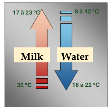
Schematic diagram of the pre-cooler principle
